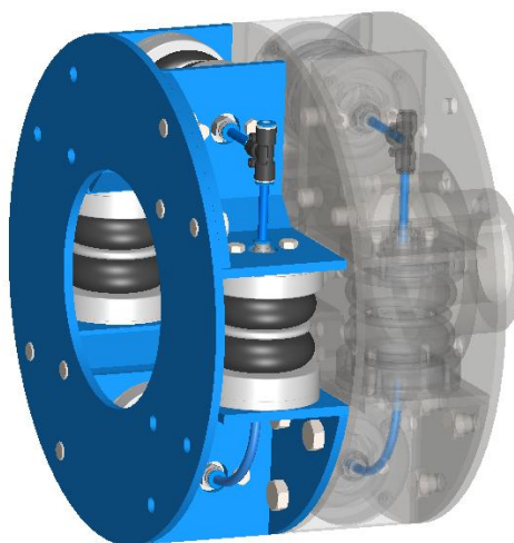
Fig. 1 Redistributor of vibration energy - 3D model
