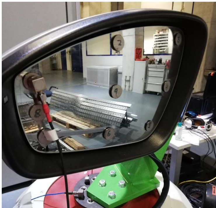
Fig. 1 Measurement of operating waveforms of rearview mirror oscillations
