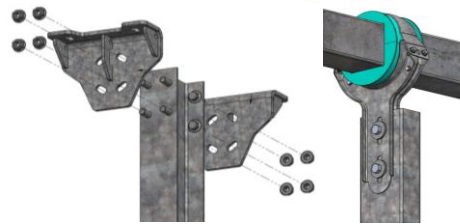
Fig. 2. Washer Joints are Used for the Assembly of these structures very Often.
