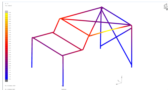
Fig.1 Deformations of the Steel Frame.
