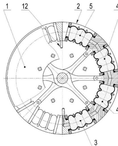
Fig. 1 Pneumatic flexible chain shaft coupling
